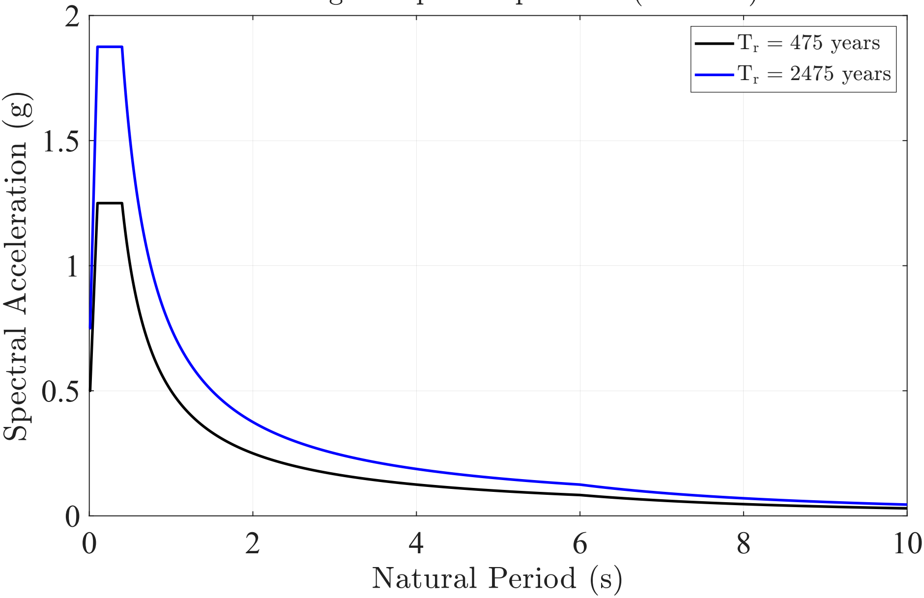
IS Design Response Spectrum (Zone VI)
